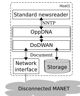
Figure 4. Architecture of an OppDNA instance
